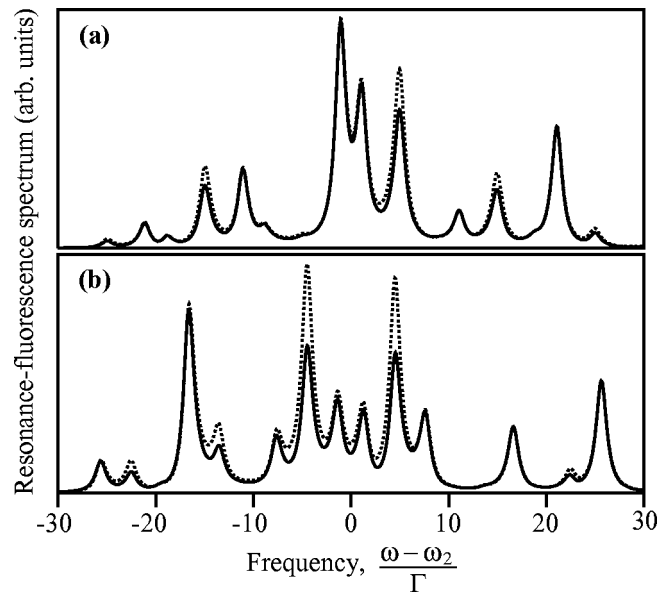
FIG. 1. Discrepancies in the predictions of the resonance-fluorescence spectrum, with (a) \delta = 5\Gamma , \Delta = 0 , \Omega_1 = 8\Gamma , and \Omega_2 = 13.6\Gamma [originally investigated in Ref. [2], Fig. 4(c)], and (b) \delta = 9\Gamma/2 , \Delta = -11\Gamma/2 , \Omega_1 = 8\Gamma , and \Omega_2 = 16\Gamma . Solid lines show the predictions from Ref. [1], and dashed lines show those from Ref. [2]. Note that Ref. [1] computes the inelastic fluorescence spectrum and Ref. [2] computes the total fluorescence spectrum; these spectra should agree everywhere except for frequencies \omega = \omega_2 - 2l\delta (for integer l ), which correspond to the locations of the spikes in the elastic spectrum. We have omitted these frequencies in these plots.
