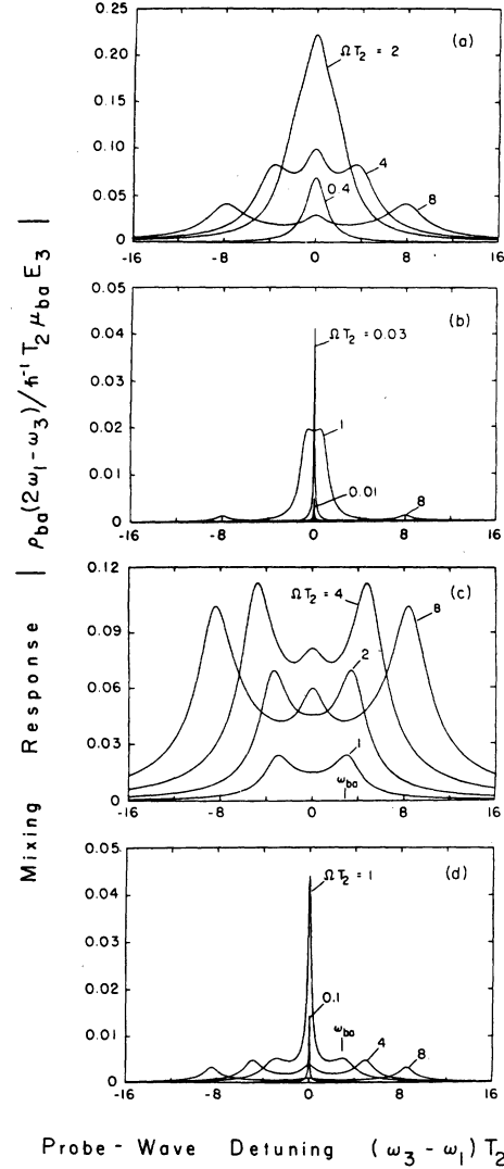
FIG. 10. The modulus of the mixing response is shown as a function of the probe-wave detuning for the following cases: (a) (\omega_1 - \omega_{ba})T_2=0 , T_2/T_1=2 ; (b) (\omega_1 - \omega_{ba})T_2=0 , T_2/T_1=0.02 ; (c) (\omega_1 - \omega_{ba})T_2=-3 , T_2/T_1=2 ; (d) (\omega_1 - \omega_{ba})T_2=-3 , T_2/T_1=0.02 .
